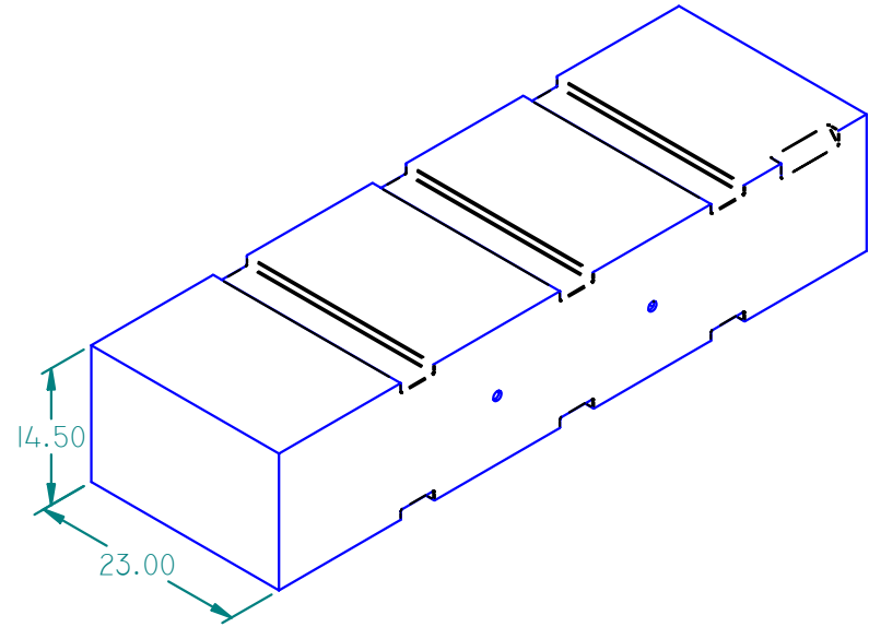
ISO VIEW 120100
